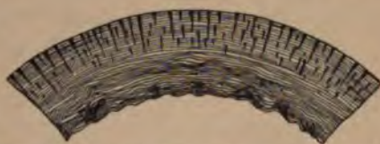
FIG. 26. — A bent stratum to illustrate tension upon the convex and compression upon the concave side (after Van Hise).
